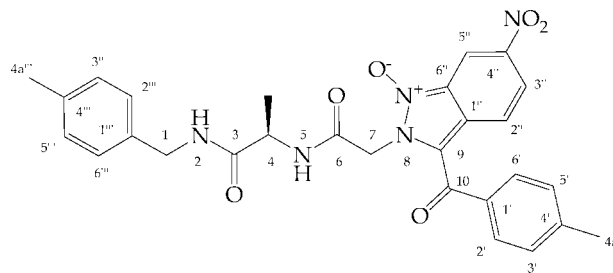
FIGURE 1. Atom numbering of compound 6(8,2,1) .
